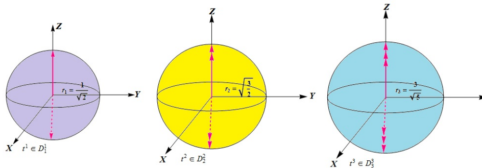
Figure: Multiaxial representation of t^1 , t^2 and t^3 characterizing the W state.
