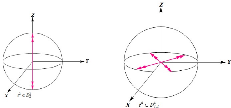
Figure: Multiaxial representation of t^2 and t^4 characterizing the GHZ state.
