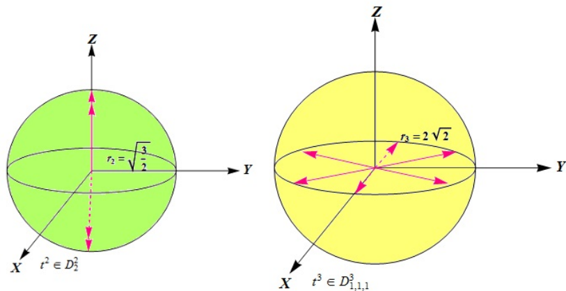
Figure: Multiaxial representation of t^2 and t^3 characterizing the GHZ state.
